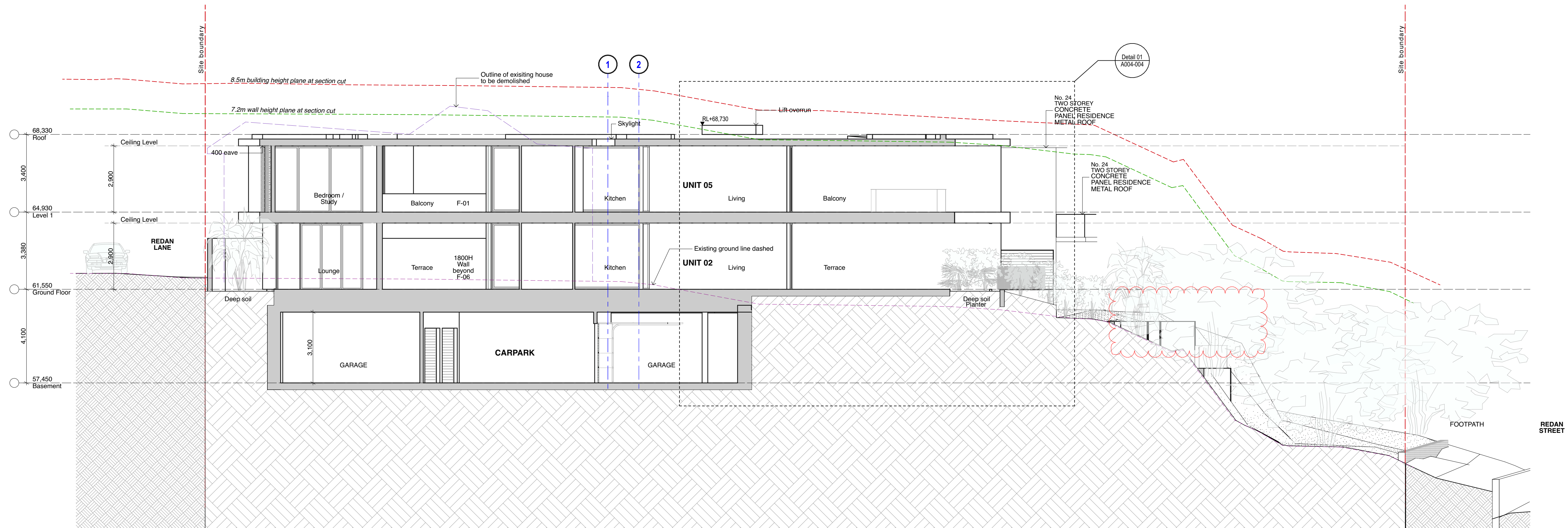
SECTION A/A
