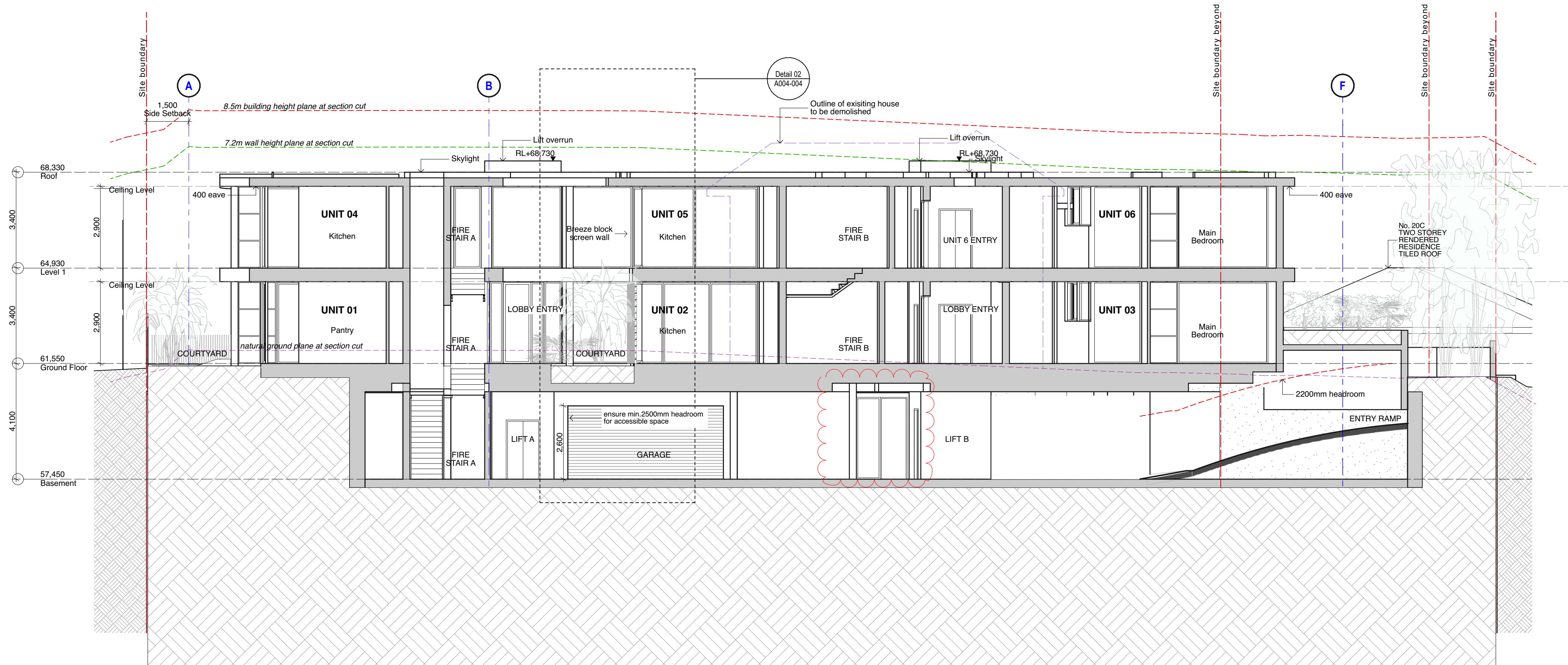
SECTION B/B
